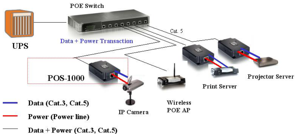
POE-1000 Product Diagram
